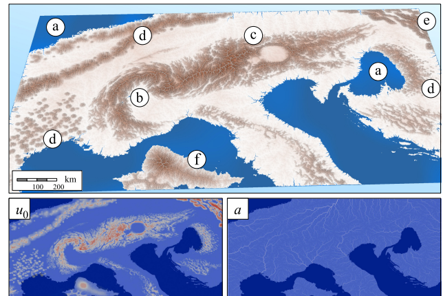
Fig. 23. Authoring of a large terrain (about 1,200 × 600 km), starting from an inverse procedural modeling of the Alps, and using several high-level brushes to edit existing features and add new ones: (a) sea editing, (b) twist deformation, (c) erase brush to create craters, (d) point primitives distribution, (e) low frequency warping, and (f) sketching of a replica of O’ahu island in the Mediterranean sea.
